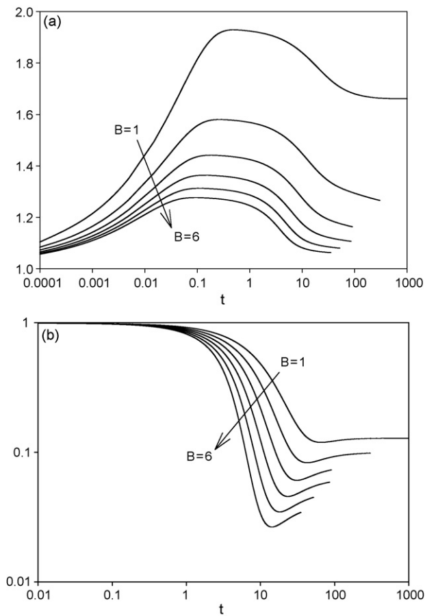
Fig. 9. Effects of the Bingham number B on (a) the length of the yielded domain and (b) the coherency parameter at the rotating surface; a_0 = a_1 = a_2 = 0.01 and n = 0.5 .
