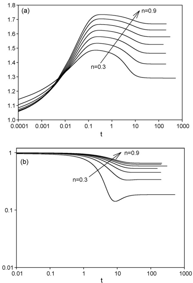
Fig. 13. Effects of n on (a) the length of the yielded domain and (b) the coherency parameter at the rotating surface; B = 2 , a_0 = 0.1 , a_1 = a_2 = 0.01 .
